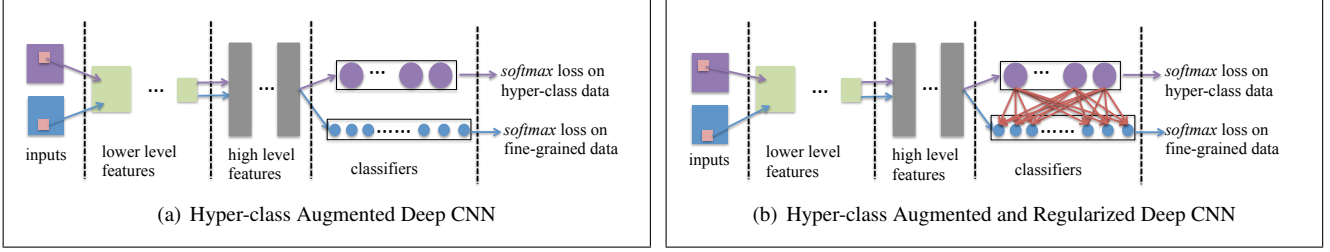
Figure 4. The network structures.
