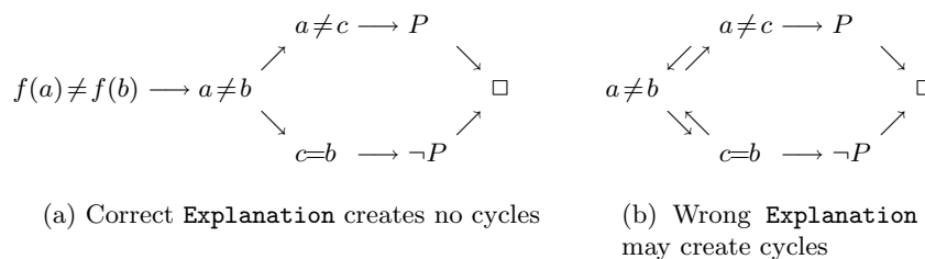
Fig. 1. Creation of undesirable cycles in the implication graph.
