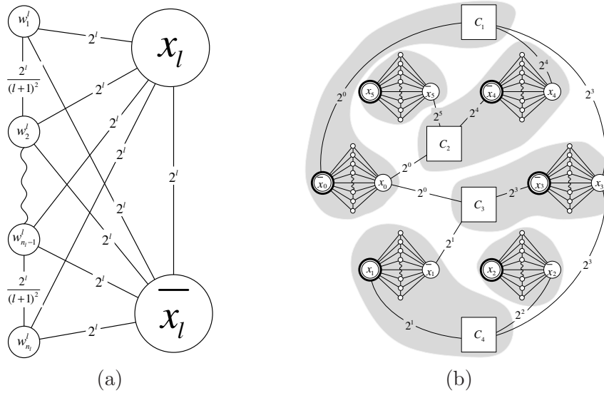
Figure 2: (a) The gadget for the variable x_l in \Phi . Each edge between w_i^l and w_{i+1}^l has weight exactly 2^l / (l + 1)^2 and the number of w_i^l 's is 8(l + 1)^2 + 1 . (b) A representation of an instance of k -clustering on a doubling metric constructed from an instance of \Phi . All “clause-literal” edges have weight 2^l for variable x_l . The optimal cover is highlighted with grey “blobs”. \Phi = (\neg x_0 \vee x_3 \vee x_4) \wedge (x_0 \vee \neg x_4 \vee \neg x_5) \wedge (x_0 \vee \neg x_1 \vee \neg x_3) \wedge (x_1 \vee \neg x_2 \vee x_3) . Satisfying assignment X = (0, 1, 1, 0, 0, 1) . Weight of the covering is exactly 2^6 - 1
