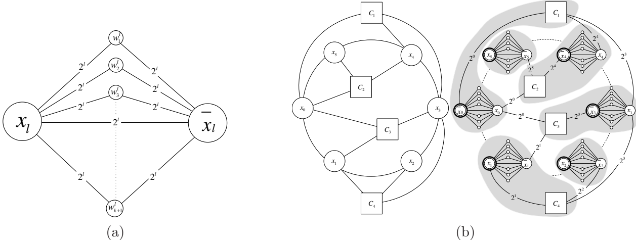
Figure 1: (a) The gadget for variable x_l in \Phi . (b) A planar embedding for \Phi and construction of the corresponding instance of k -clustering problem. All “clause-literal” edges have weight 2^l for the variable x_l . The optimal cover is highlighted with grey “blobs”. \Phi = (\neg x_0 \vee x_3 \vee x_4) \wedge (x_0 \vee \neg x_4 \vee \neg x_5) \wedge (x_0 \vee \neg x_1 \vee \neg x_3) \wedge (x_1 \vee \neg x_2 \vee x_3) . Satisfying assignment X = (0, 1, 1, 0, 0, 1) . Weight of the covering is exactly 2^6 - 1
